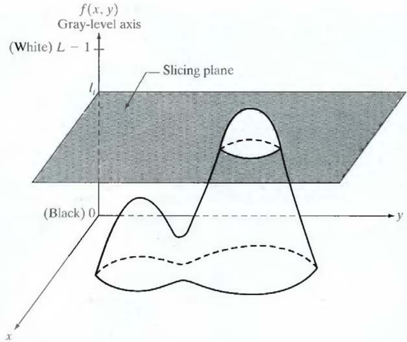
Fig 5.8.1 Geometric interpretation of the intensity-slicing technique.
